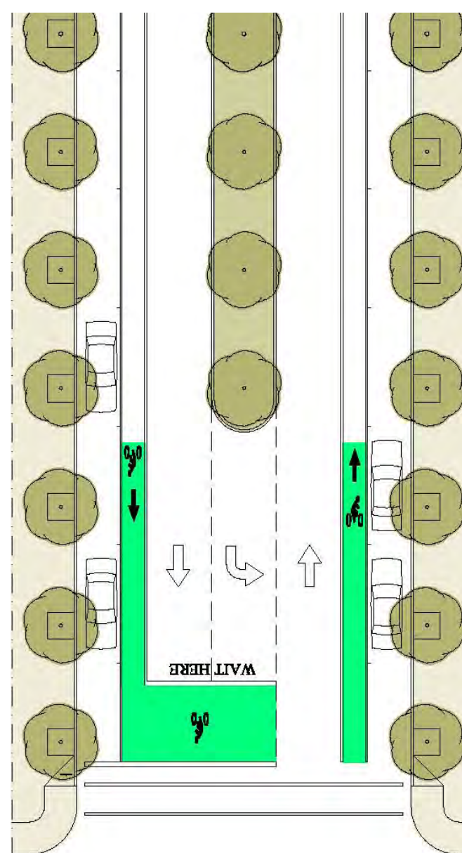
Bicycle Box
