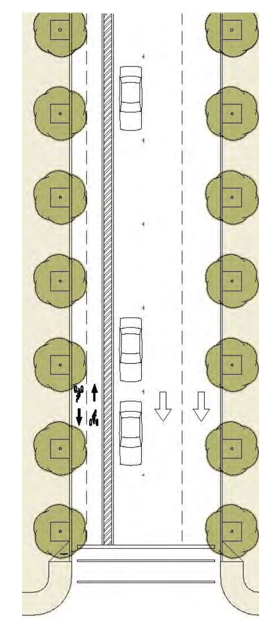
Two-Way, Physically-Separated Bicycle Lane
